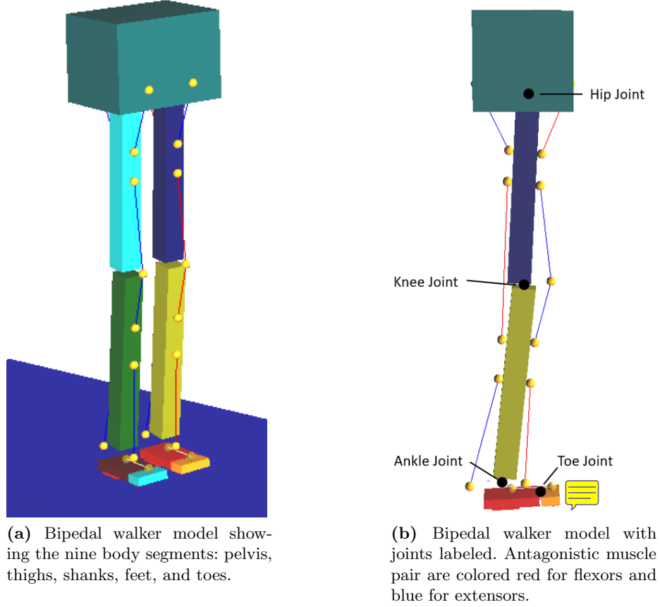
Fig. 1: Images of the bipedal walker model.
